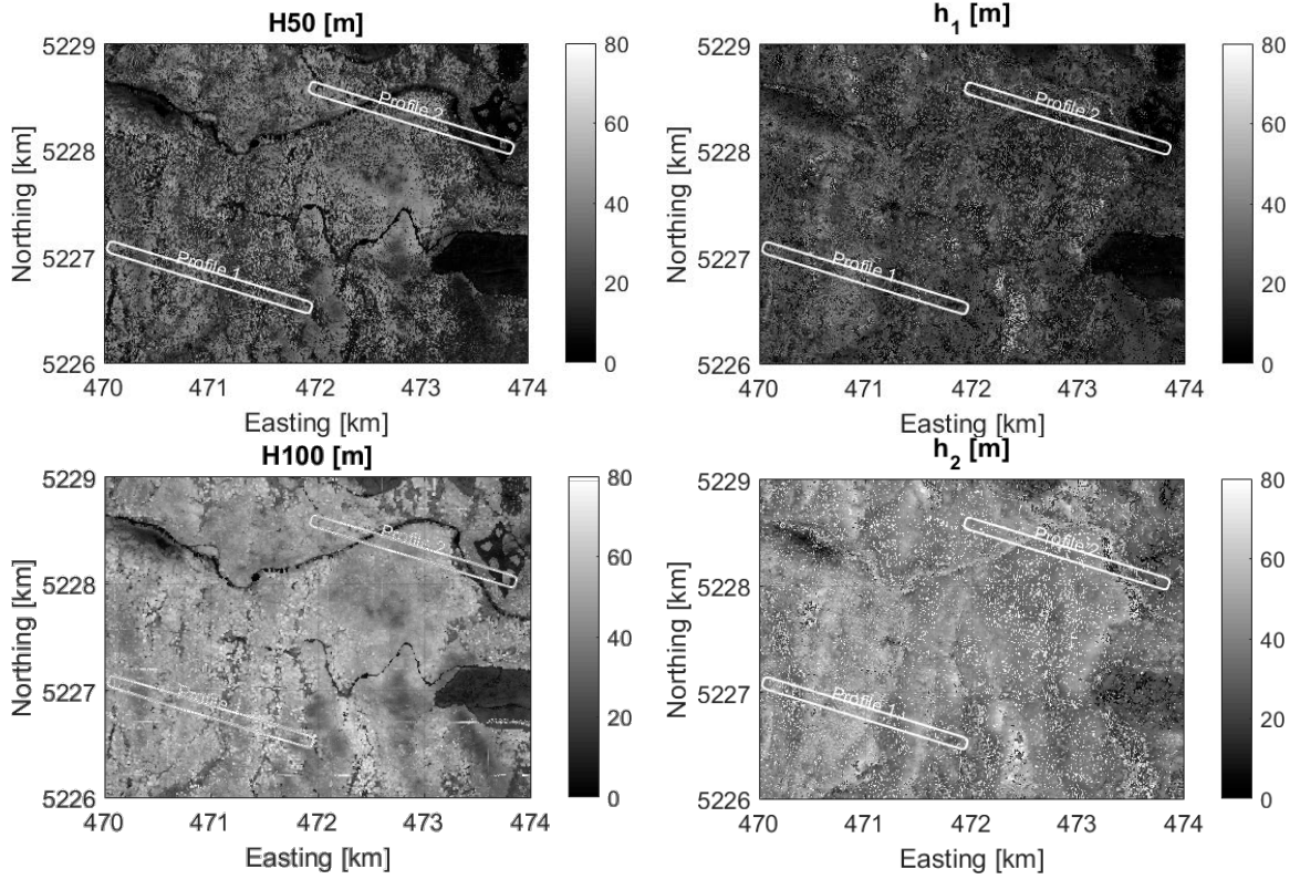
Figure 1: Comparison between H50 and H100 measured with airborne lidar scanning and h_1 and h_2 obtained from 3LM inversion of multi-temporal TanDEM-X data. All images are in UTM55N coordinates. Profile 1 is in the south-western part of the area and profile 2 is in the north-eastern part of the area.
